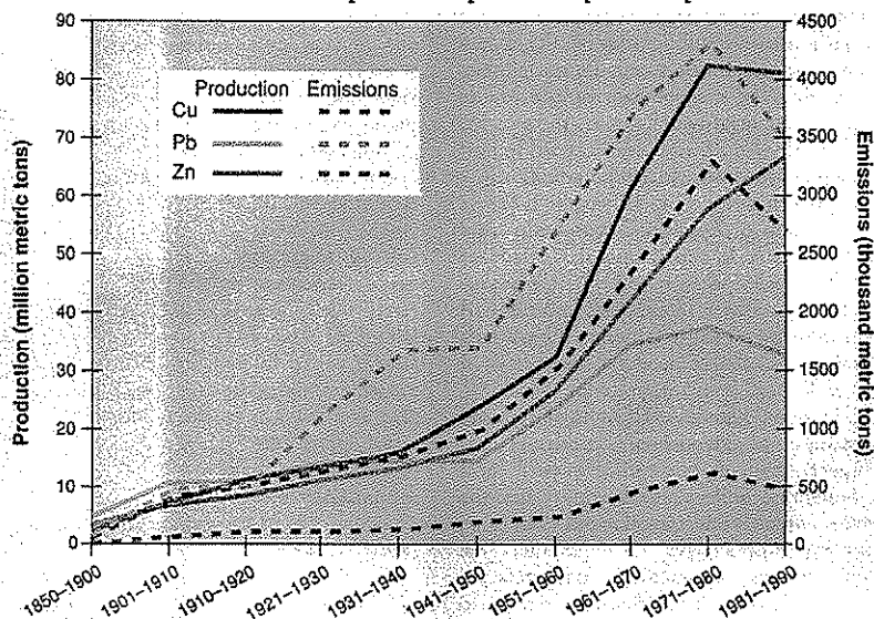
Recent historical changes in mine production and anthropogenic emissions of trace metals to the atmosphere [revised from (5)].
